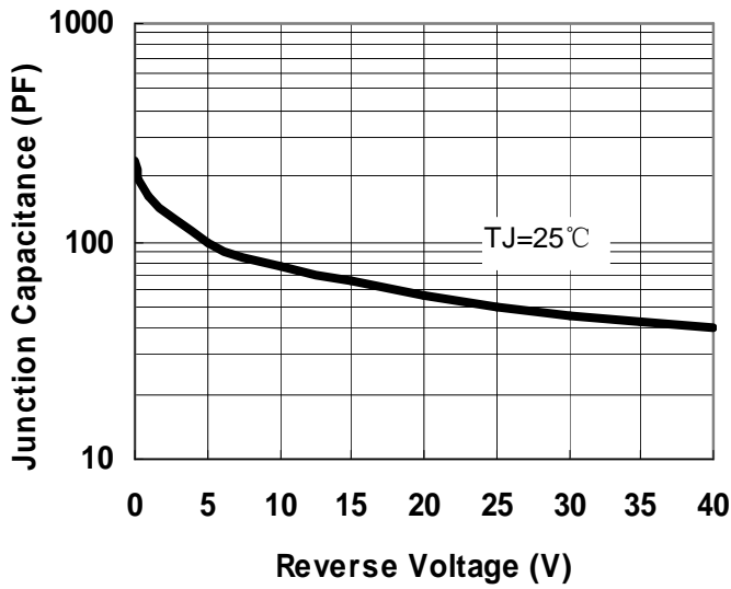
Fig.1-Typical Junction Capacitance
